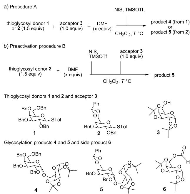
Scheme 2. a) First DMF-modulated glycosylation procedure (procedure A). b) Second DMF-modulated glycosylation procedure (procedure B). Bn = benzyl, Tol = p -tolyl.
